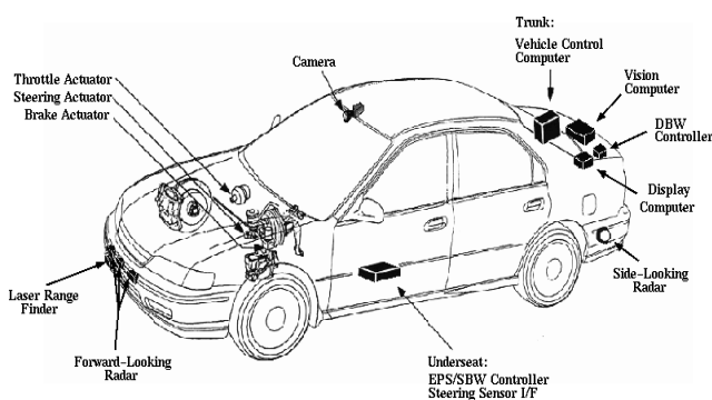
Fig. 8. OSU Autonomous Vehicle [21]
