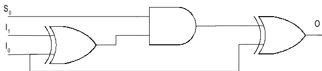
Fig. 4. GA generated 2-to-1 multiplexer
